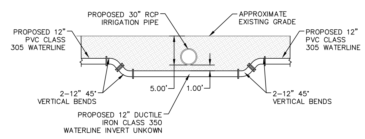
CROSSING DETAIL "D" SCALE: 1"=10'
