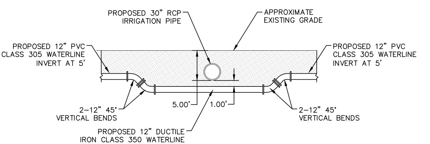
CROSSING DETAIL "A" SCALE: 1"=10'
