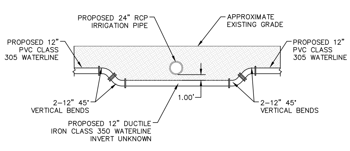
CROSSING DETAIL "B" SCALE: 1"=10'
