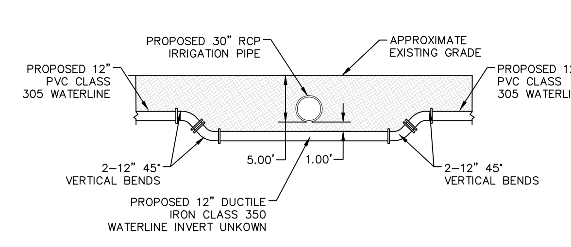
CROSSING DETAIL "C" SCALE: 1"=10'
